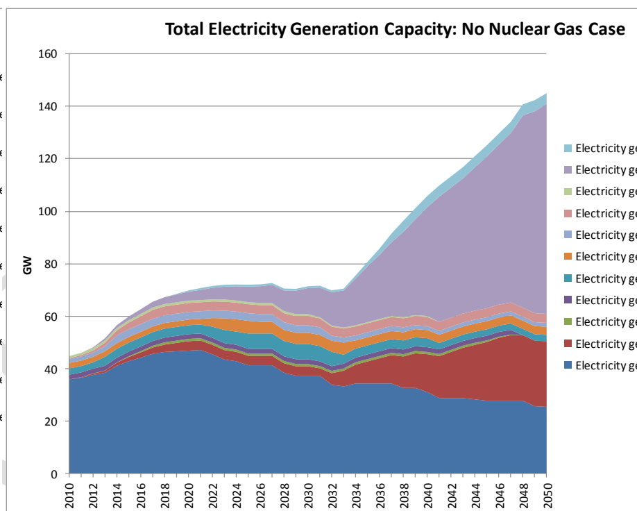
Figure 7-4: Electricity generation capacity: Emissions Limit – Natural Gas Case
