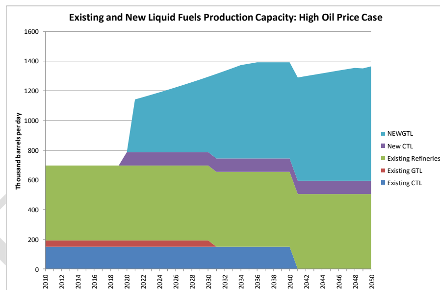
Figure 7-11: Total capacity in liquid fuel production: High Oil Price Case
