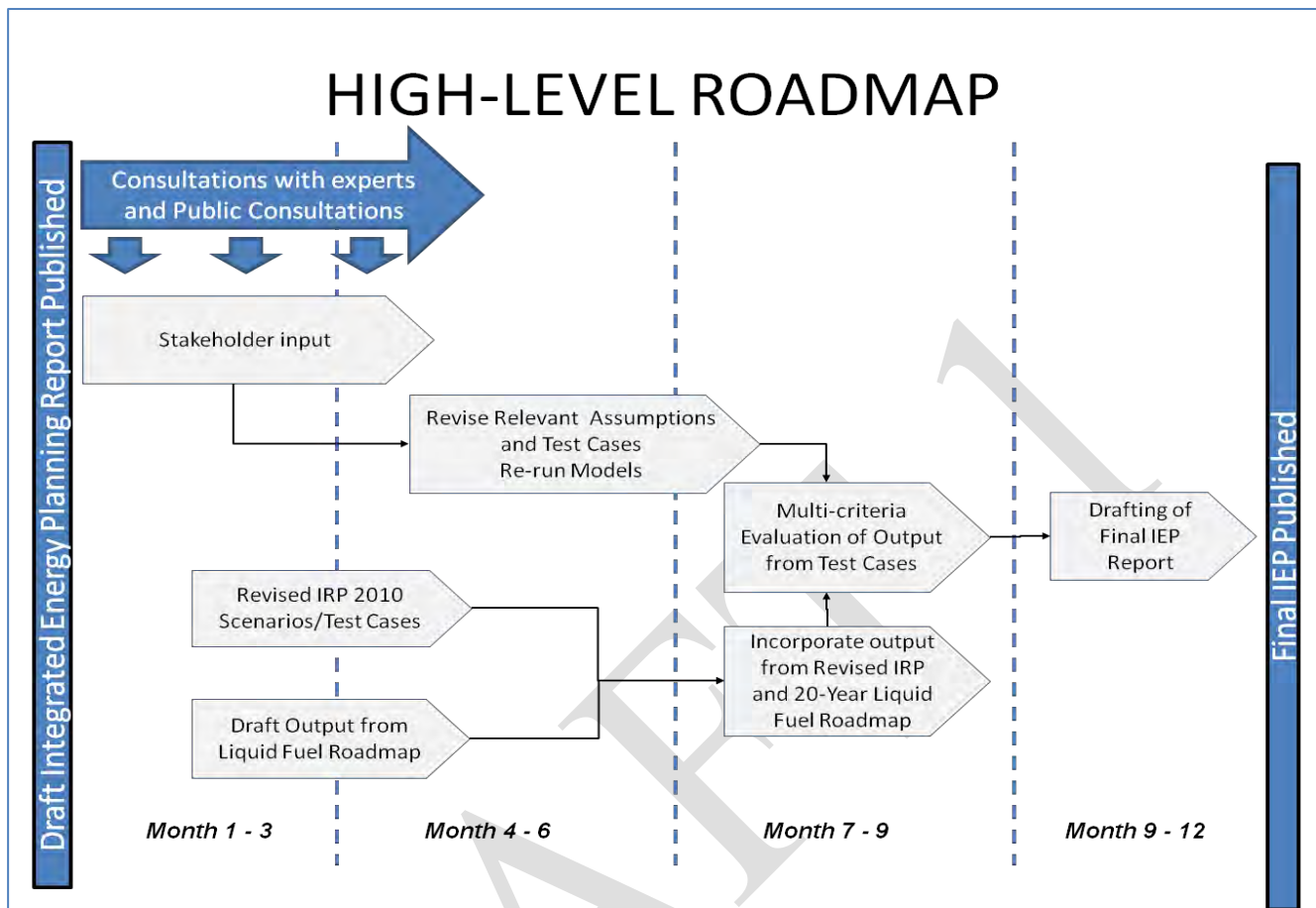
Figure 0-11: High-level roadmap
