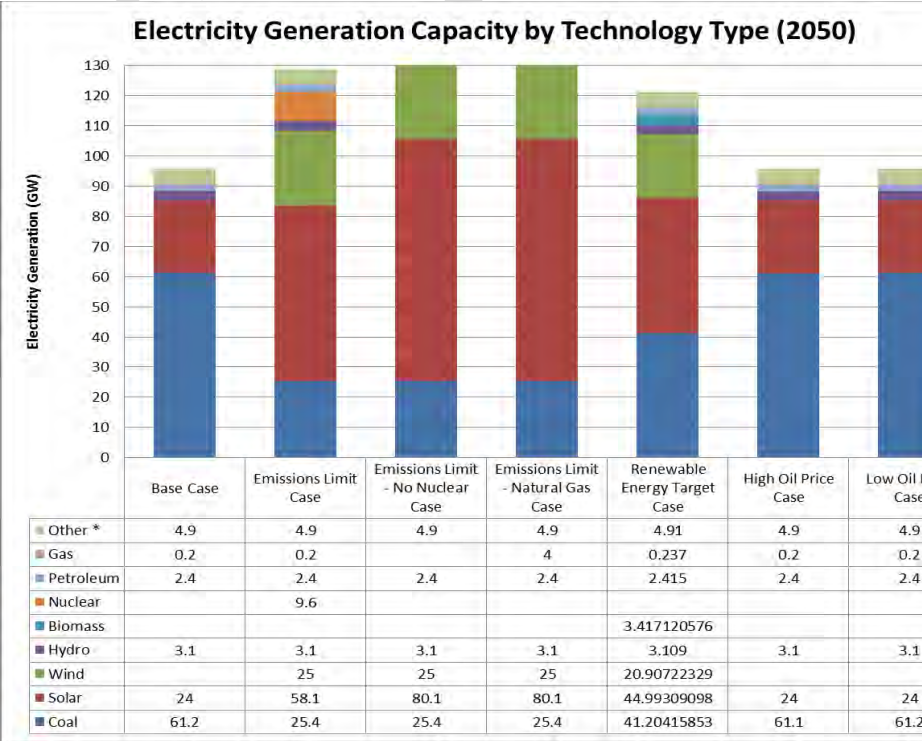
Figure 7-7: Electricity generation capacity by technology type (2050)
