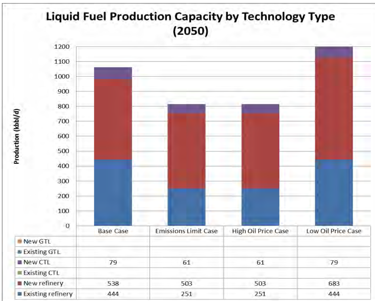
Figure 0-7: Liquid fuel production by technology type (2050)
