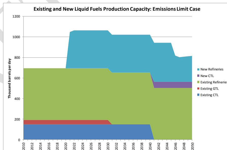
Figure 7-9: Total capacity in liquid fuel production: Emission Limit Case
