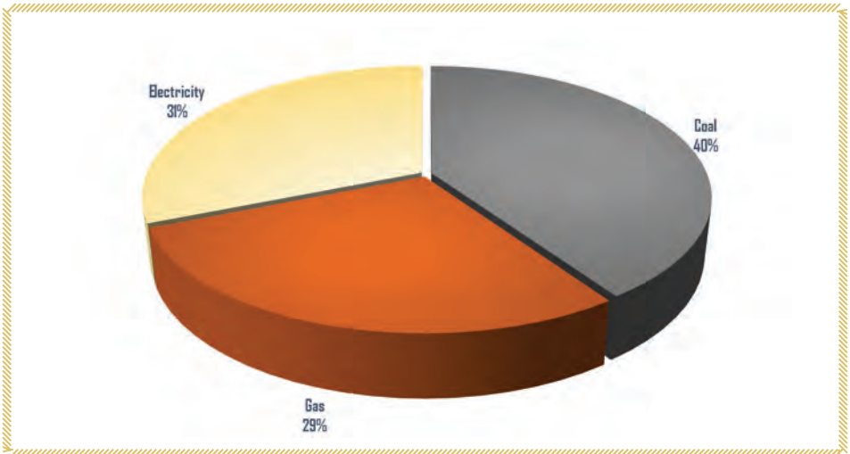
Figure 2.5: Energy demand in Iron and Steel industry, 2019
