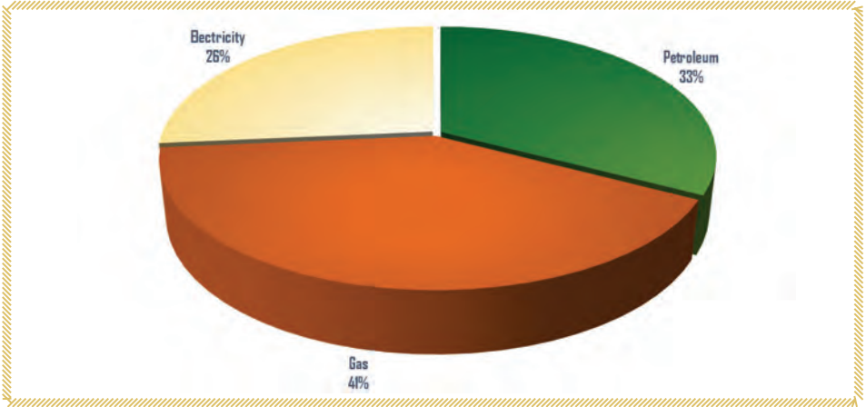
Figure 2.9: Energy demand in food and tobacco, 2019
