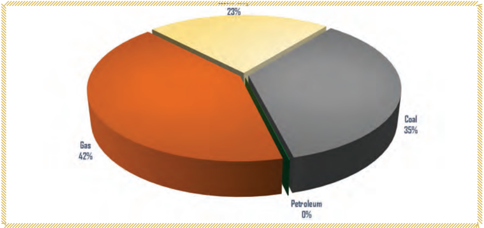
Figure 2.6: Energy demand in Chemical and Petrochemical industry, 2019
