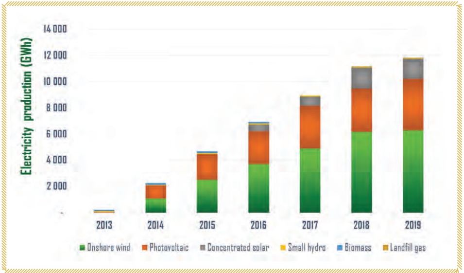
Figure 1.11: Electricity production through REIPPPP, 2013 - 2019
