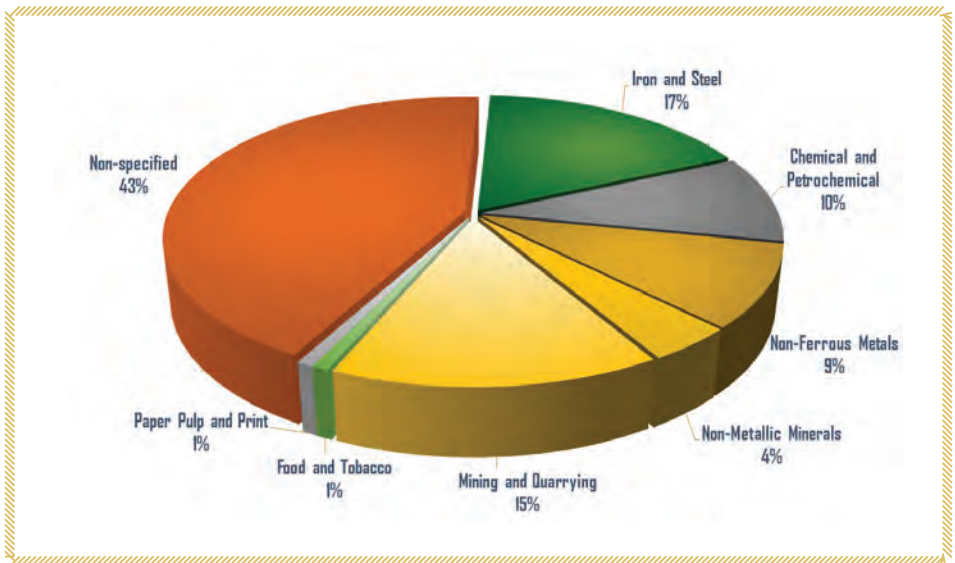
Figure 2.2: Energy demand by industrial sub-sectors, 2019
