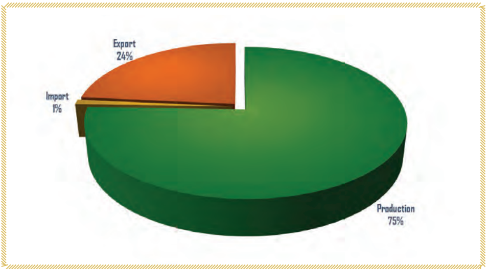
Figure 1.9: Coal primary supply, 2019
