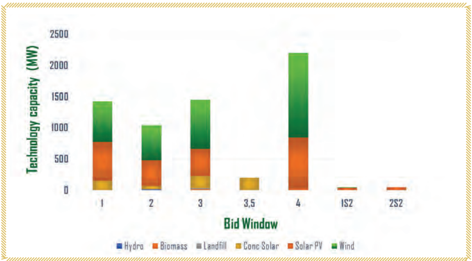
Figure 1.10: Programme capacity in windows 1, 2, 3 and 4
