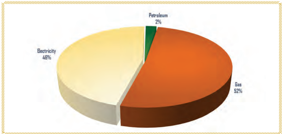
Figure 2.10: Energy demand in pulp and paper, 2019
