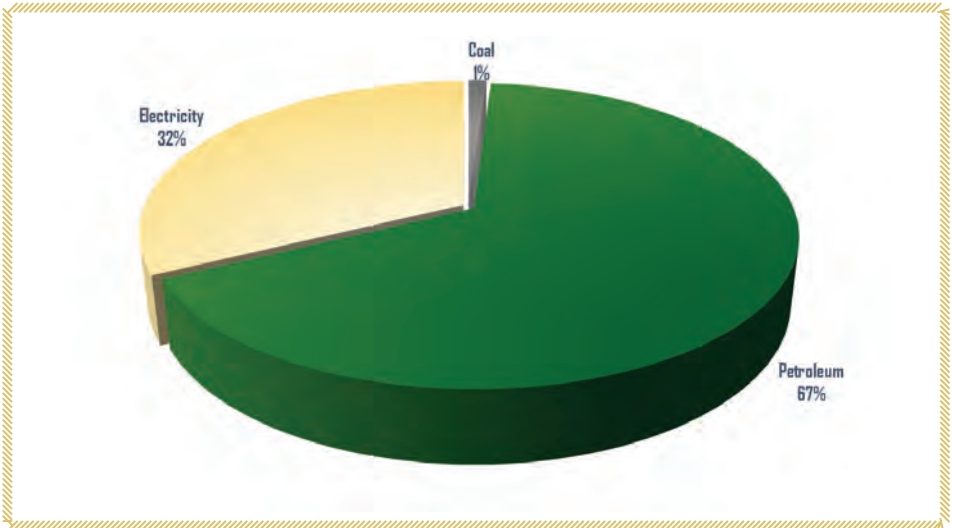
Figure 2.12: Energy demand in the agriculture sector, 2019
