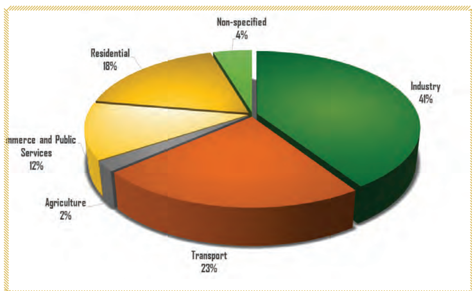
Figure 2.1: Energy demand by sector, 2019
