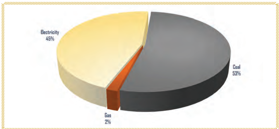
Figure 2.7: Energy demand in non-ferrous metals, 2019
