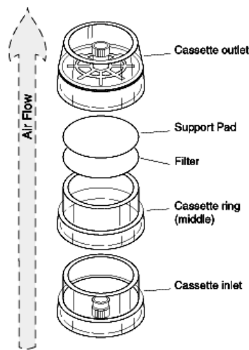
Figure D1: Filter assembly
